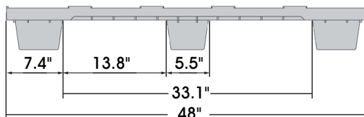
LONG SIDE VIEW
