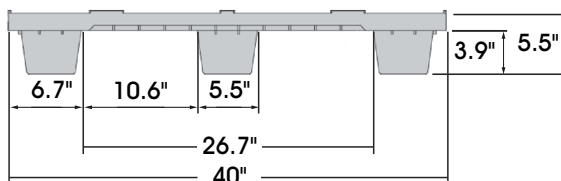
SHORT SIDE VIEW
